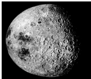
the far side of the Moon
